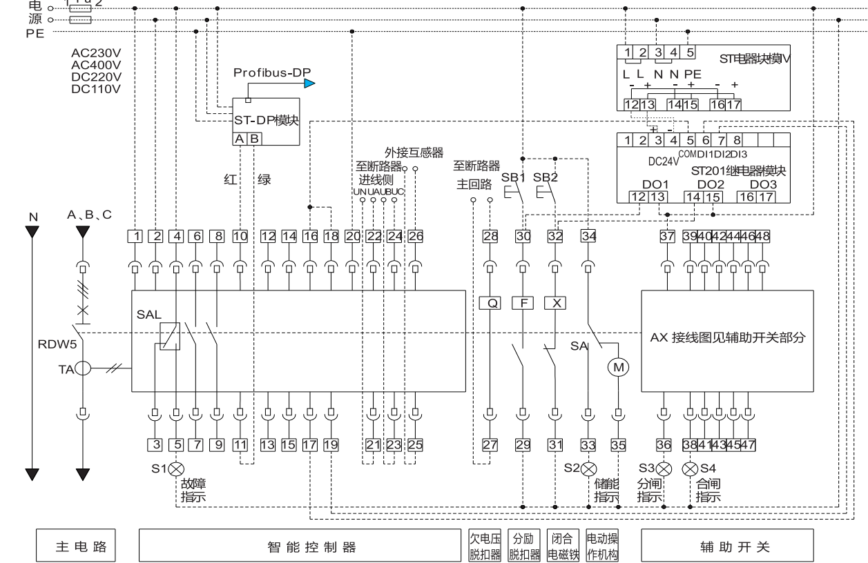
RDW5-1000S/H,1600S,2000~6300S/H H型二次回路接线图
