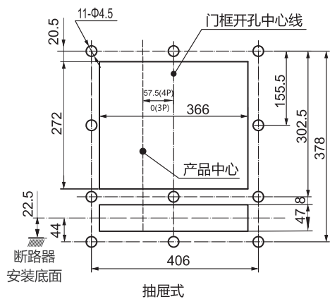
RDW5-4000S抽屉式断路器面板开孔尺寸
