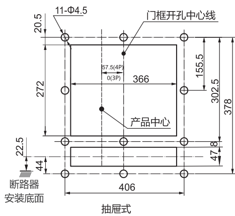
RDW5-3200S抽屉式断路器面板开孔尺寸
