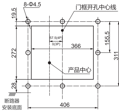
RDW5-3200H固定式断路器面板开孔尺寸
