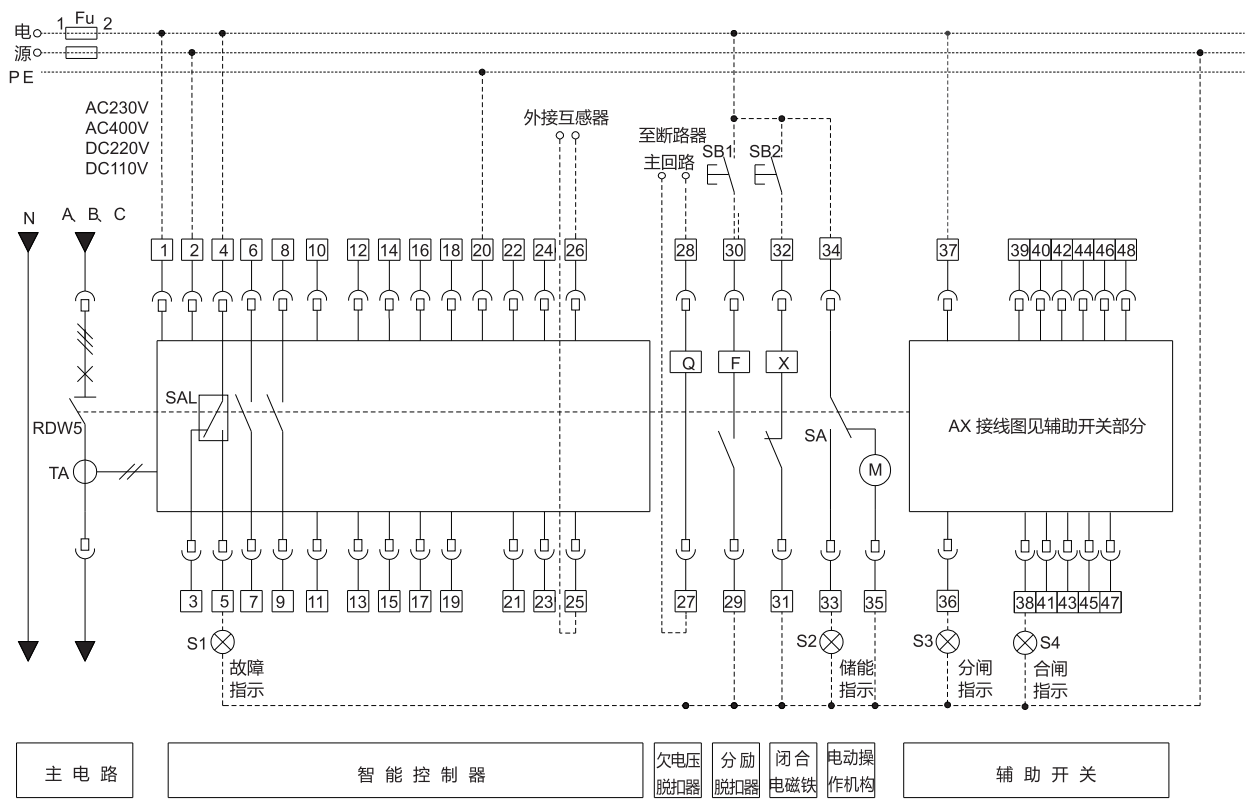
RDW5-1000S/H,1600S,2000~6300S/H M型二次回路接线图
