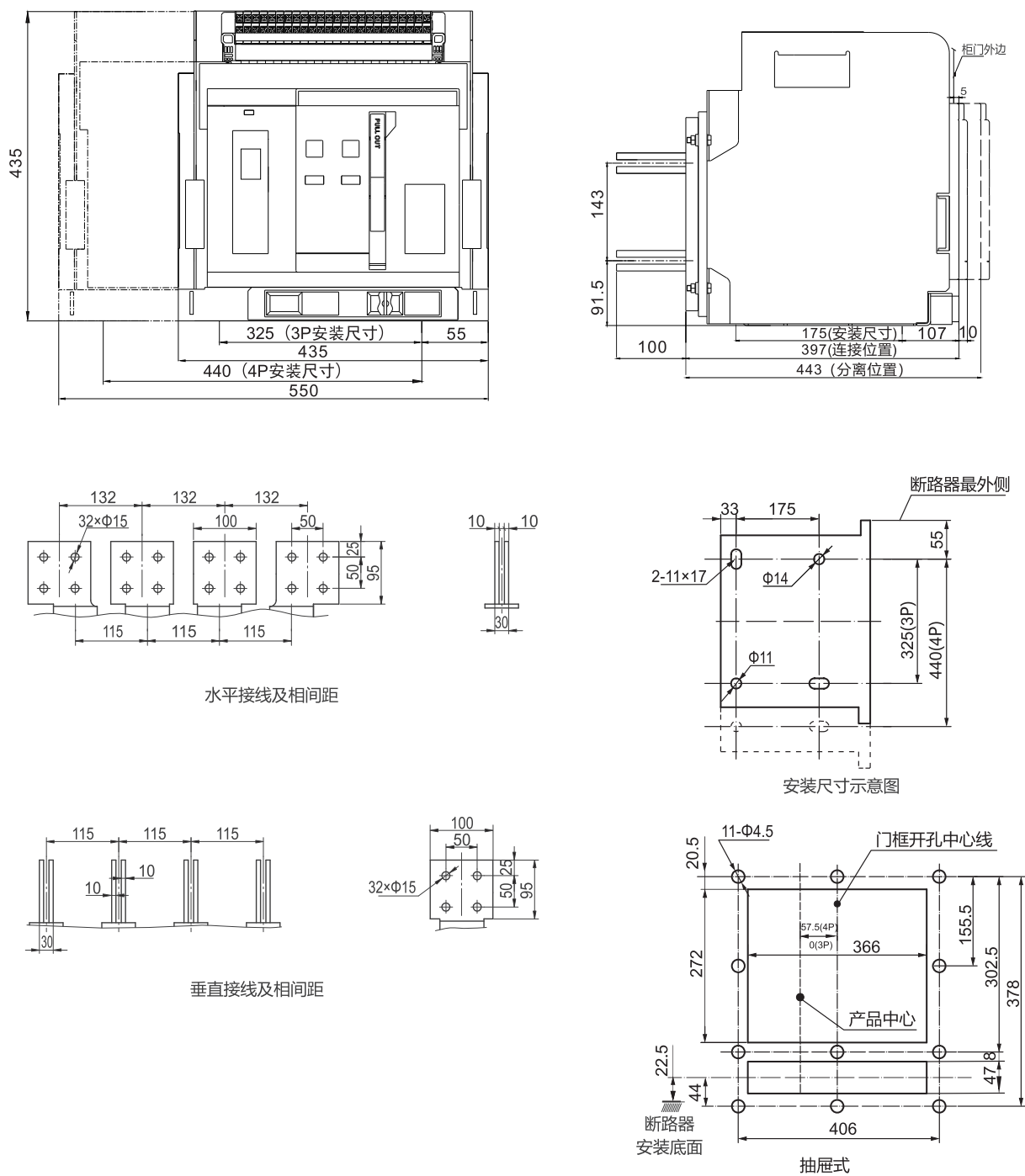
RDW5-4000H抽屉式断路器面板开孔尺寸
