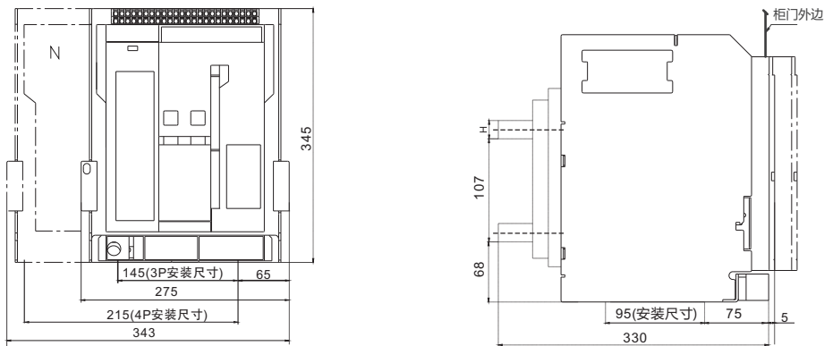
RDW5-1000S/H~1600S安装尺寸
