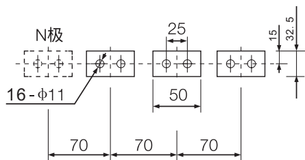
RDW5-1000S/H~1600S接线尺寸
